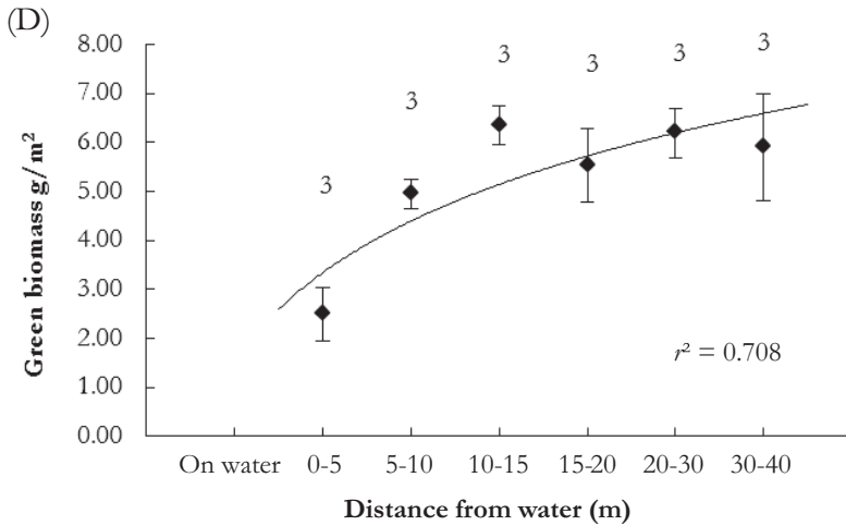
Figure 2. American Wigeon vigilance and biomass assessment in relation to distance from ephemeral waterbodies in grassland pastures near Arcata, California, USA, 31 January–24 March 2011. (A) Proportion of time vigilant (mean \pm s.e.) for American Wigeon foraging on water, and at progressively further distances from a water source ( y = 0.0324x + 0.0074 , r^2_{119} = 0.974 , P < 0.001 ). (B) Rate of “head-ups” (mean \pm s.e.) while foraging on water and at progressively further distances from water ( y = 0.059\ln(x) + 0.0508 , r^2_{119} = 0.906 , P < 0.001 ). (C) Scanning duration (length of individual head-ups) in relation to distance from water ( y = 0.1427x + 0.5345 , r^2_{119} = 0.908 , P < 0.001 ). (D) Amount of green biomass per m^2 (mean \pm s.e.) available to grazing American Wigeon at different distances from water ( y = 0.139\ln(x) + 0.2605 , r^2_{21} = 0.763 , P < 0.01 ).
